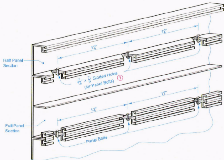
ASSEMBLY DETAIL
